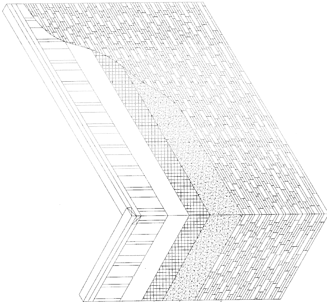
TYPICAL INTERIOR STUD WALL
