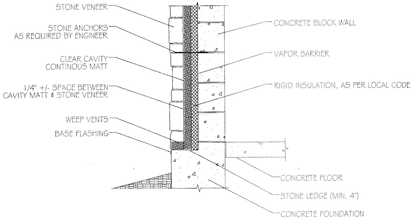
TYPICAL SECTION FOR CLEAR CAVITY CONCRETE FOUNDATION WALL
