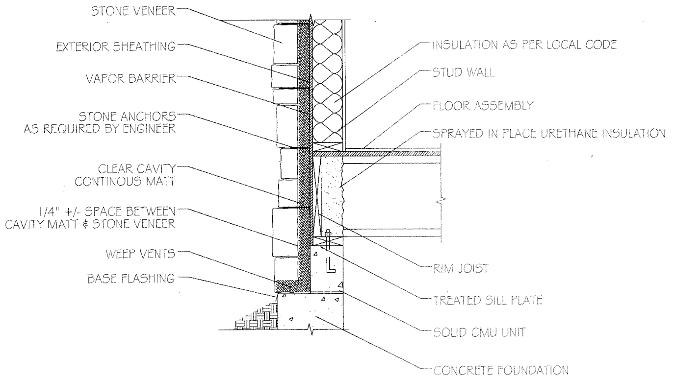
TYPICAL SECTION FOR CLEAR CAVITY STUD WALL
